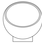
F5 Diffuser Ø 450 mm D 300 mm Base Ø 200 mm H 60 mm
