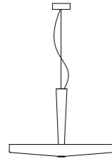
S3 - S33 Ceiling Rose Ø 120 mm Cable 3555 mm Diffuser Ø 680 mm H 445 mm
